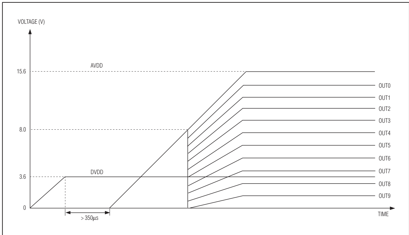
Figure 13. Power-Up Sequence
